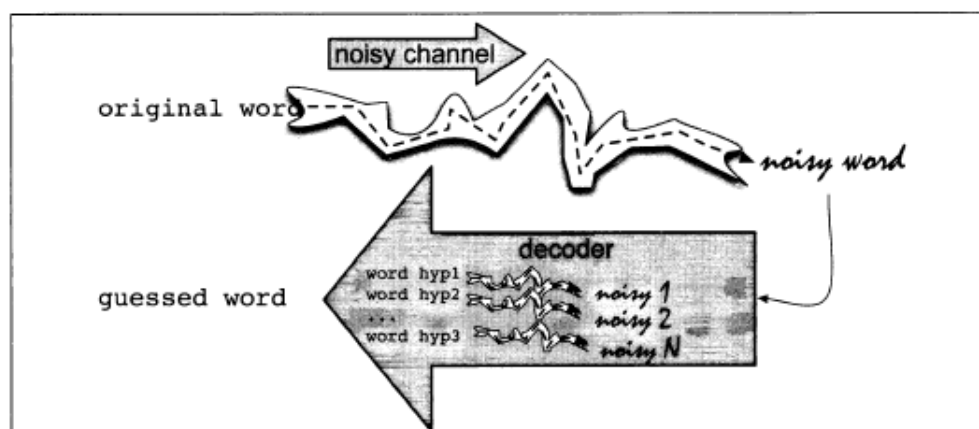
Figure 5.23 In the noisy channel model, we imagine that the surface form we see is actually a “distorted” form of an original word passed through a noisy channel. The decoder passes each hypothesis through a model of this channel and picks the word that best matches the surface noisy word.
