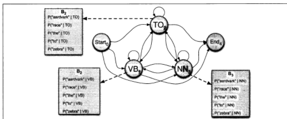
Figure 5.14 The B observation likelihoods for the HMM in the previous figure. Each state (except the non-emitting start and end states) is associated with a vector of probabilities, one likelihood for each possible observation word.
