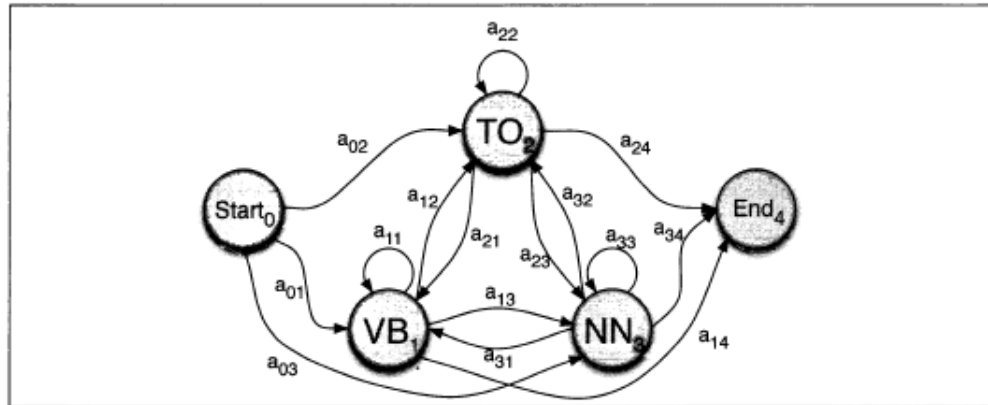
Figure 5.13 The Markov chain corresponding to the hidden states of the HMM. The A transition probabilities are used to compute the prior probability.
